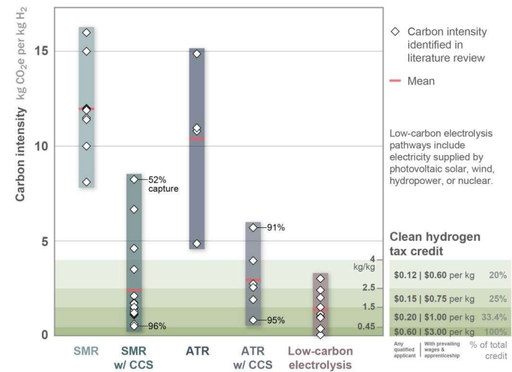
Hydrogen lifecycle carbon intensity in published literature
