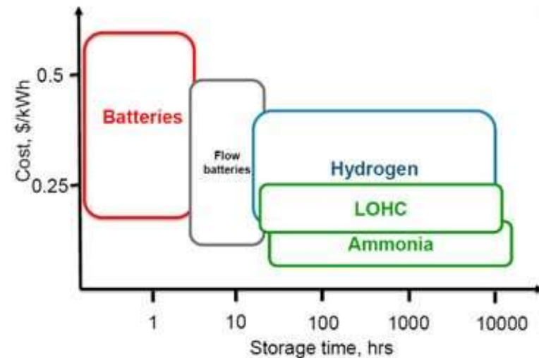
Levelized cost of energy storage
